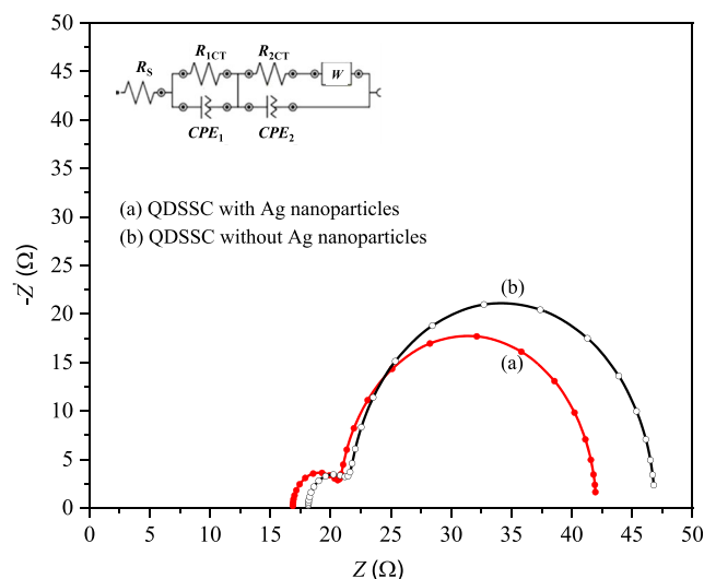
Fig. 12 Nyquist plots of PbS/CdS quantum dot-sensitized solar cells under simulated light of 100 mW cm -2 with AM 1.5 filter
